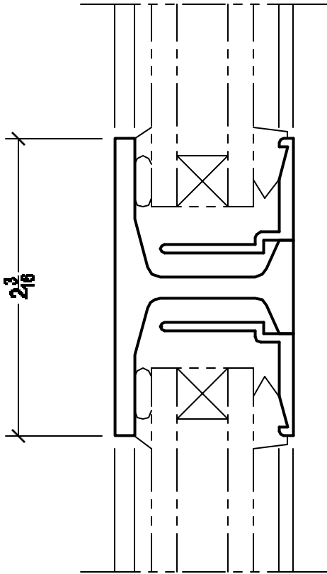
#1000M4 TRUE MUNTIN DETAIL
