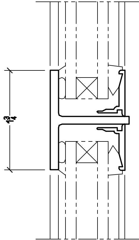
#T175 TRUE MUNTIN DETAIL
