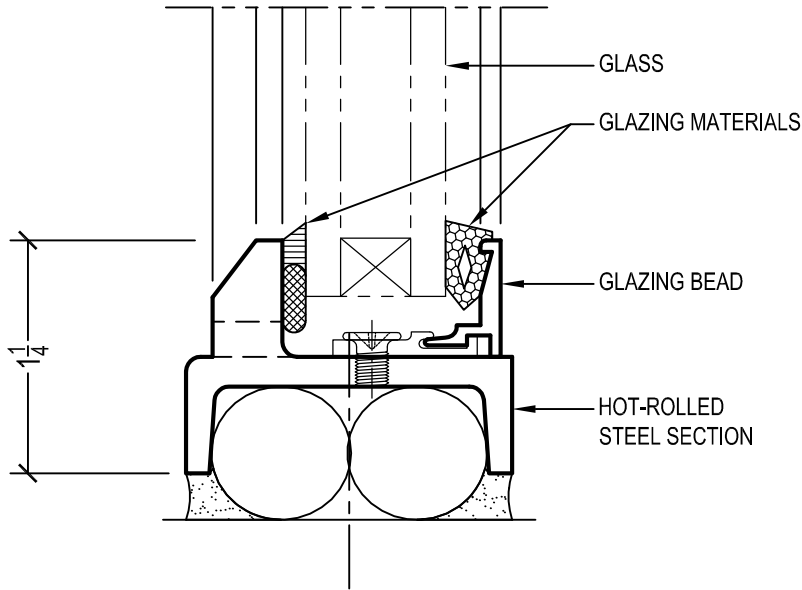
FIXED DETAIL INTERIOR GLAZED WITH 3/4" GLASS
